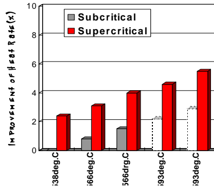
Fig.2 Heat Rate Comparison Super vs Sub Critical Conditions
