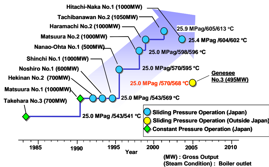
Fig.1 Trend of Steam Condition Improvement
