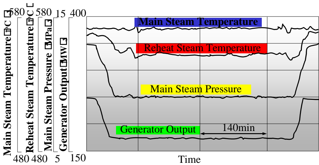
Fig.14 Result of Minimum Load Test at 35% Load
