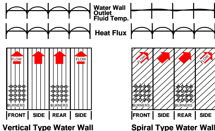
Fig.5 Spiral Wall Keeping Uniform Temperature at the Outlet
