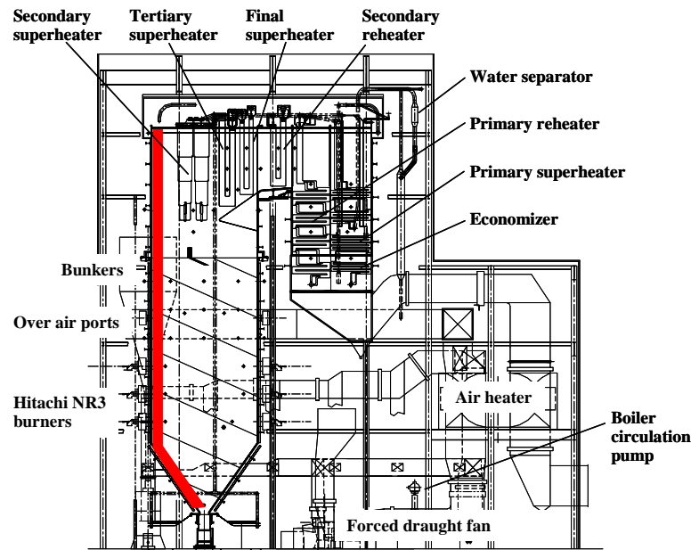
Fig. 4 Side View of Genesee Phase 3 Boiler
